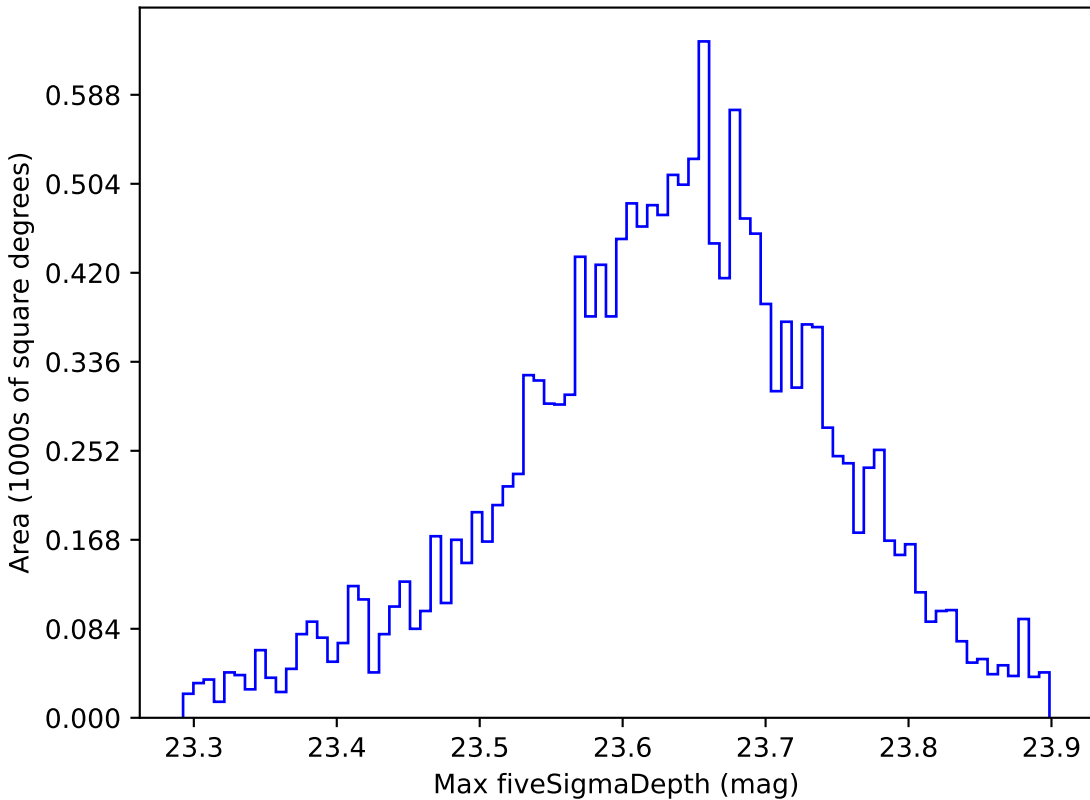
ddf_half_v3.4_10yrs WFD z band: Max fiveSigmaDepth
