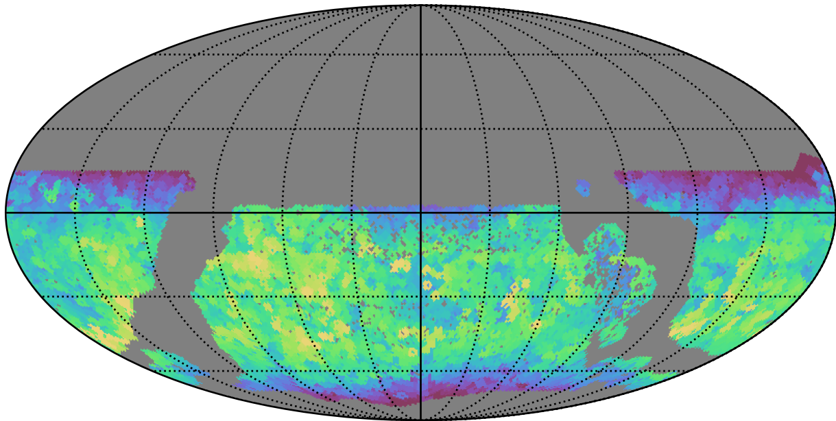
ddf_half_v3.4_10yrs WFD y band: Max fiveSigmaDepth
