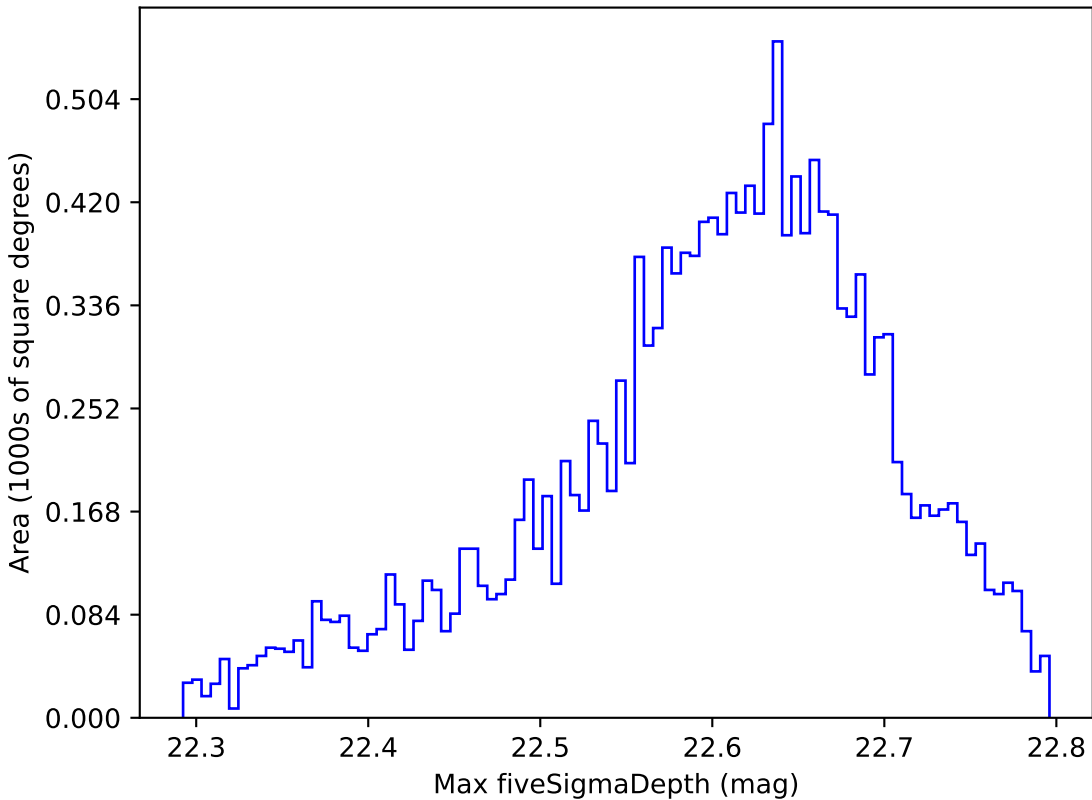
ddf_half_v3.4_10yrs WFD y band: Max fiveSigmaDepth
