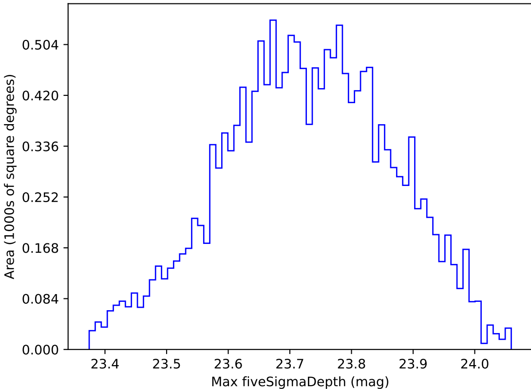
ddf_half_v3.4_10yrs WFD u band: Max fiveSigmaDepth
