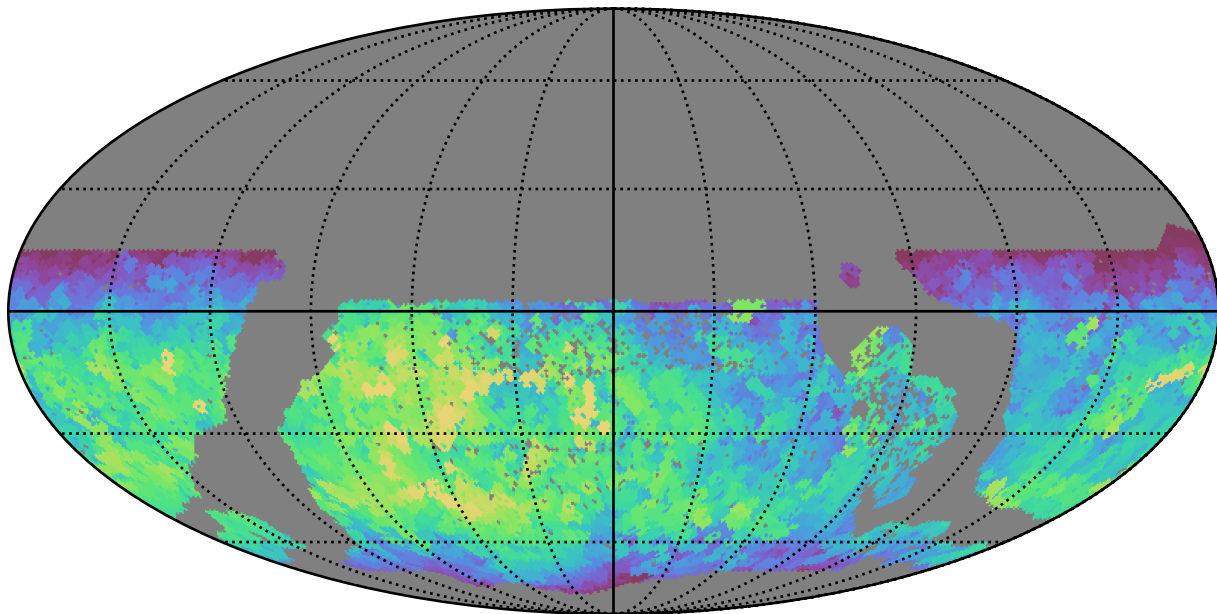
ddf_half_v3.4_10yrs WFD r band: Max fiveSigmaDepth
