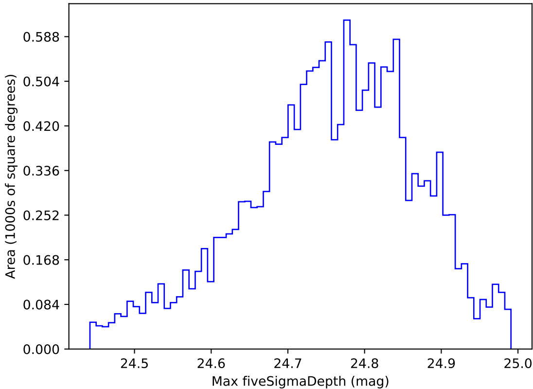
ddf_half_v3.4_10yrs WFD r band: Max fiveSigmaDepth
