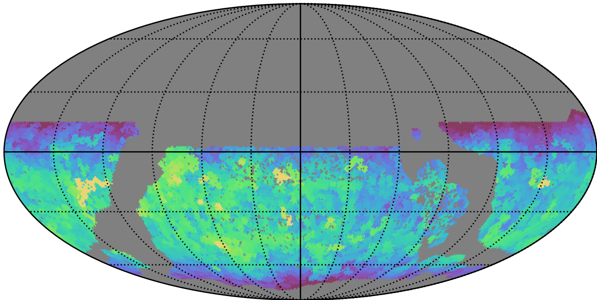
ddf_half_v3.4_10yrs WFD i band: Max fiveSigmaDepth
