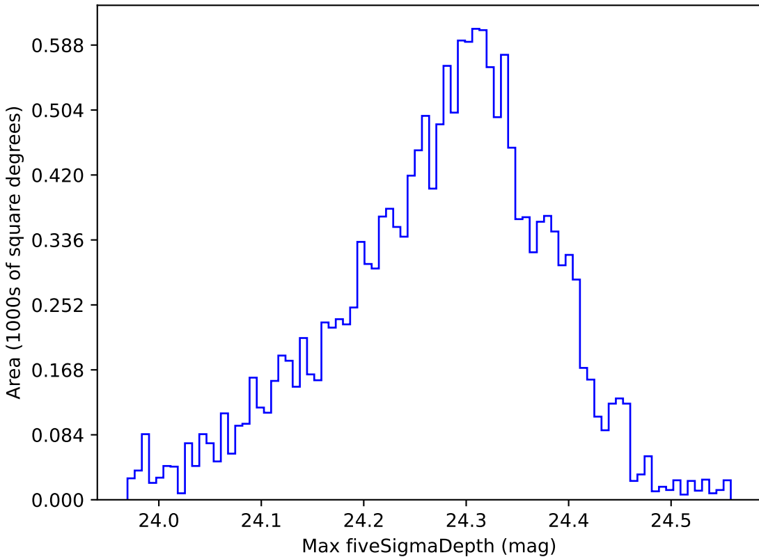
ddf_half_v3.4_10yrs WFD i band: Max fiveSigmaDepth
