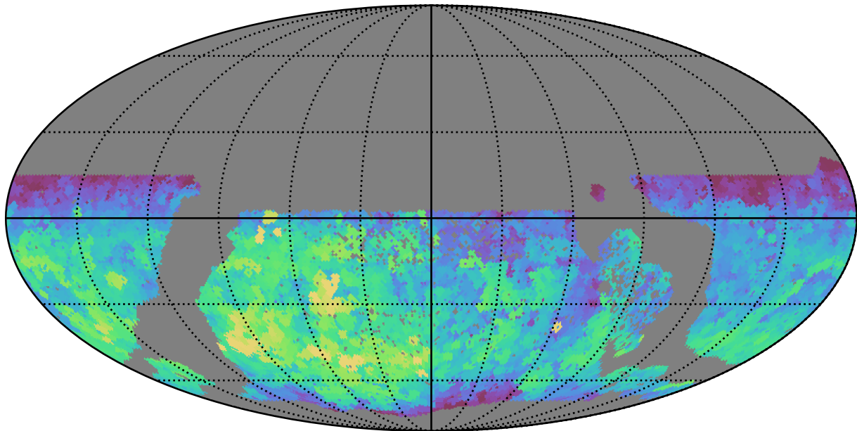
ddf_half_v3.4_10yrs WFD g band: Max fiveSigmaDepth
