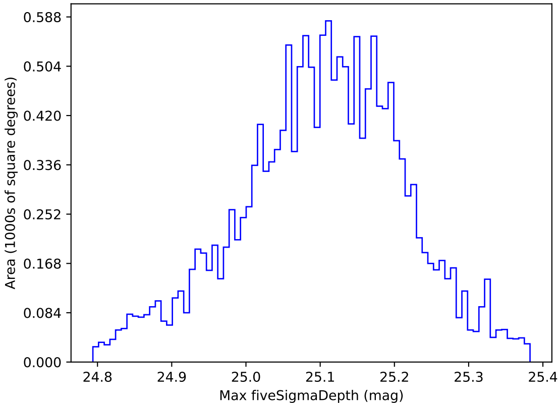
ddf_half_v3.4_10yrs WFD g band: Max fiveSigmaDepth
