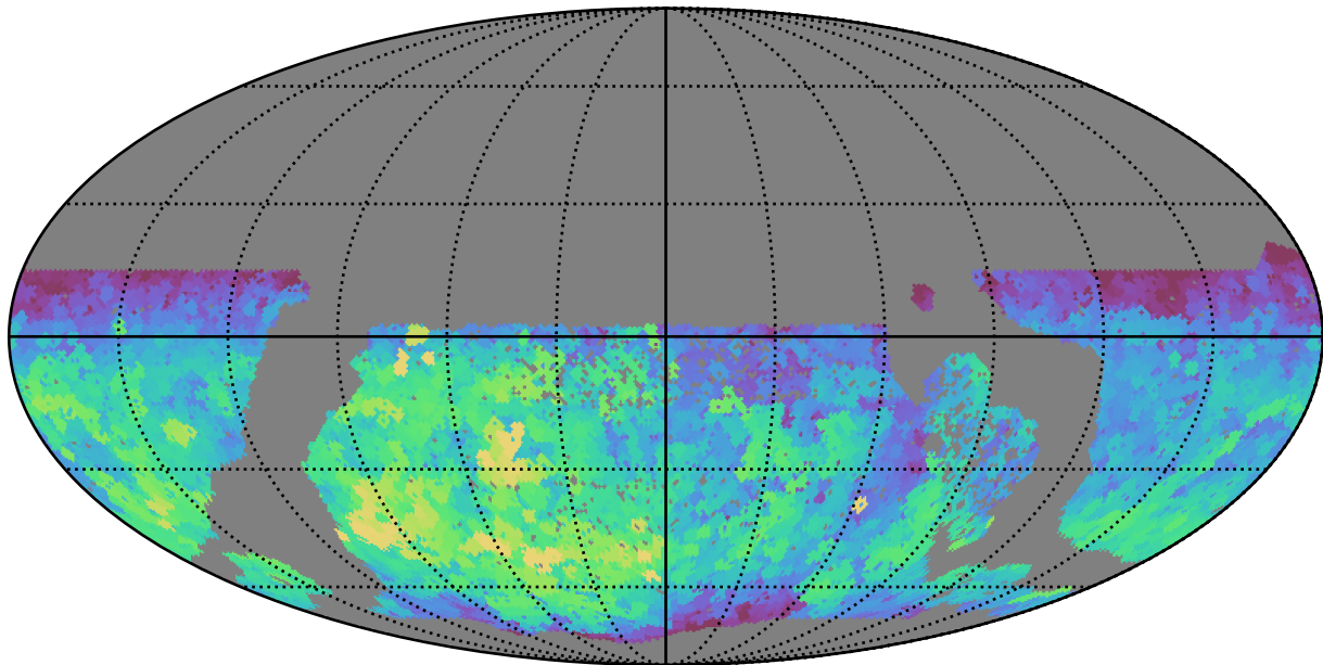
ddf_half_v3.4_10yrs WFD all bands: Max fiveSigmaDepth
