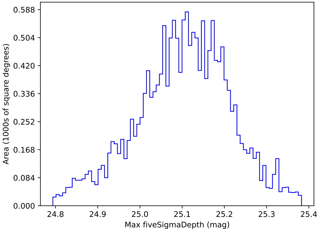
ddf_half_v3.4_10yrs WFD all bands: Max fiveSigmaDepth
