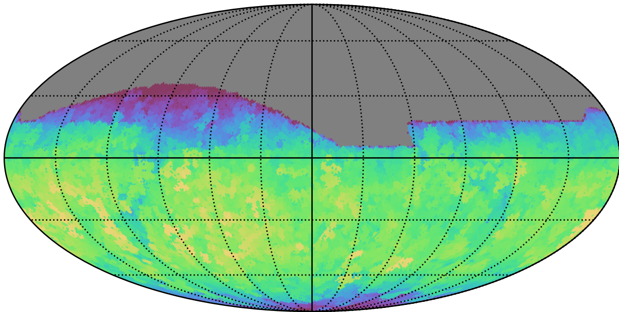
ddf_half_v3.4_10yrs All sky z band: Max fiveSigmaDepth
