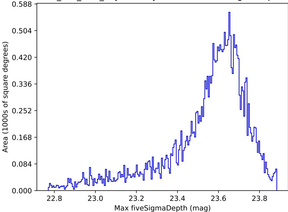
ddf_half_v3.4_10yrs All sky z band: Max fiveSigmaDepth
