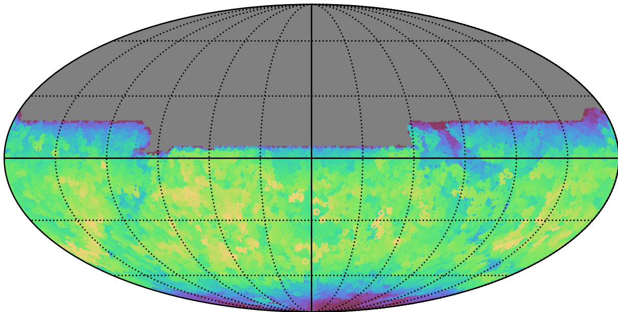
ddf_half_v3.4_10yrs All sky y band: Max fiveSigmaDepth
