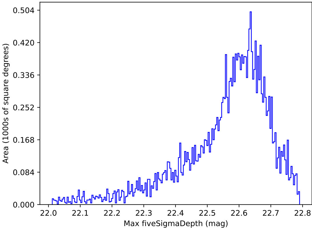
ddf_half_v3.4_10yrs All sky y band: Max fiveSigmaDepth
