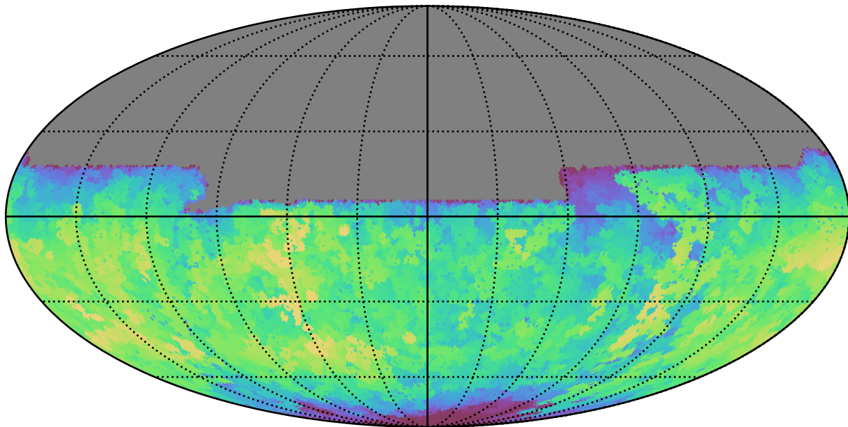
ddf_half_v3.4_10yrs All sky u band: Max fiveSigmaDepth
