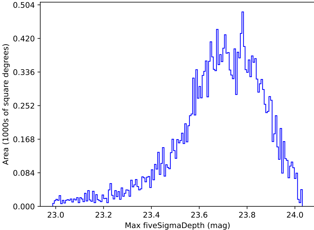
ddf_half_v3.4_10yrs All sky u band: Max fiveSigmaDepth
