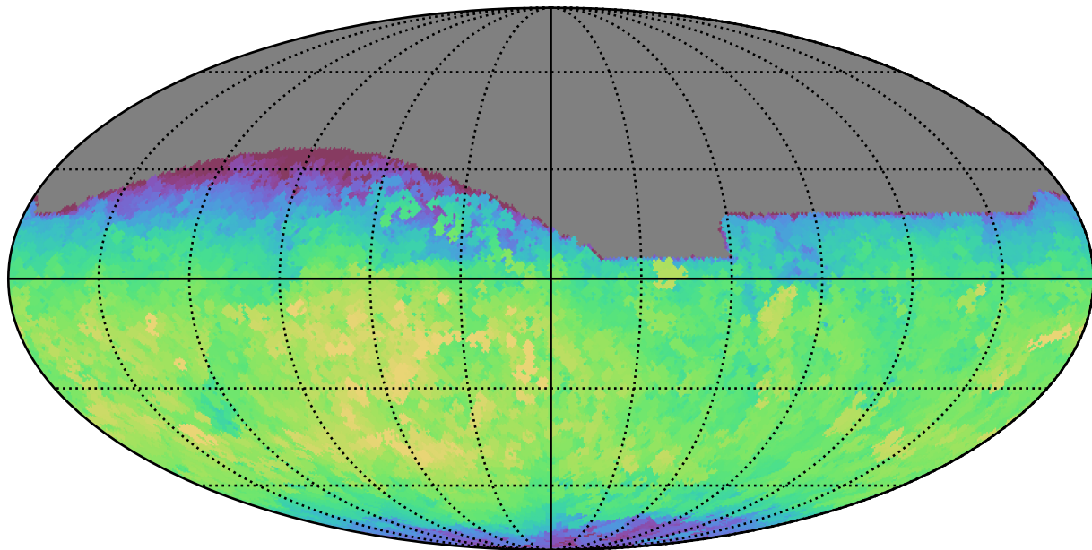
ddf_half_v3.4_10yrs All sky r band: Max fiveSigmaDepth
