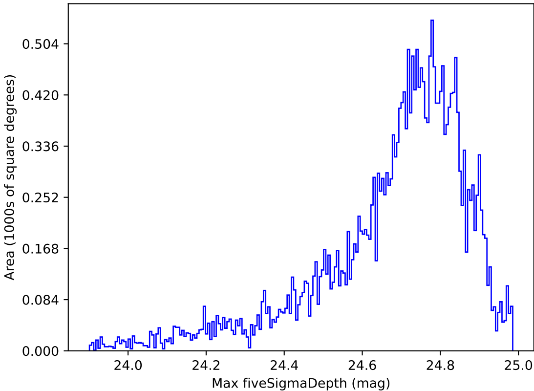
ddf_half_v3.4_10yrs All sky r band: Max fiveSigmaDepth
