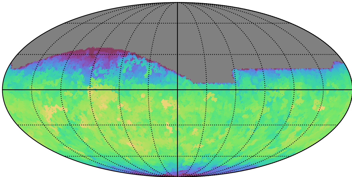
ddf_half_v3.4_10yrs All sky i band: Max fiveSigmaDepth
