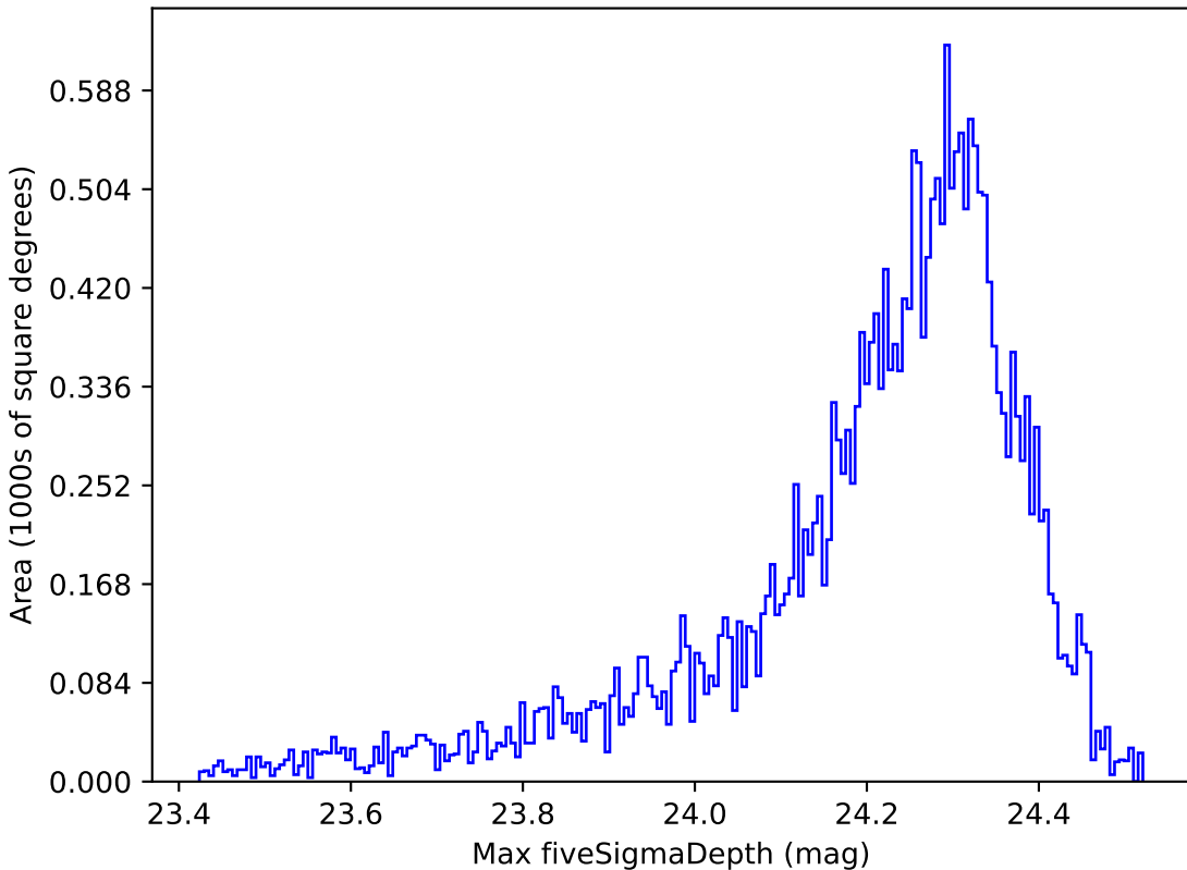
ddf_half_v3.4_10yrs All sky i band: Max fiveSigmaDepth
