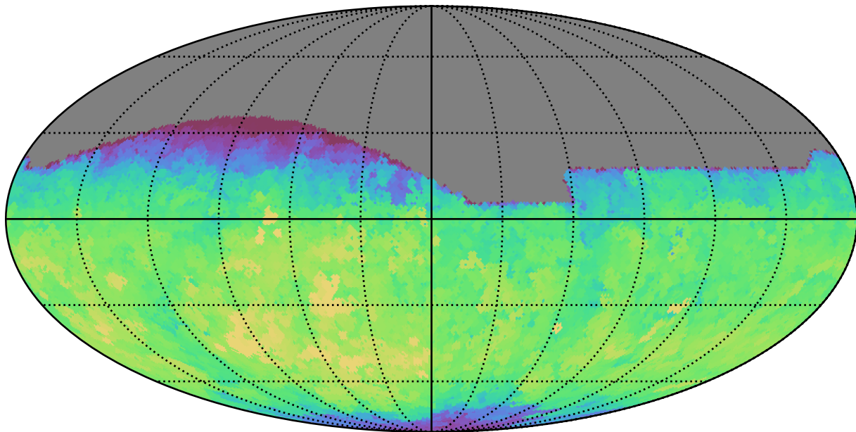
ddf_half_v3.4_10yrs All sky g band: Max fiveSigmaDepth
