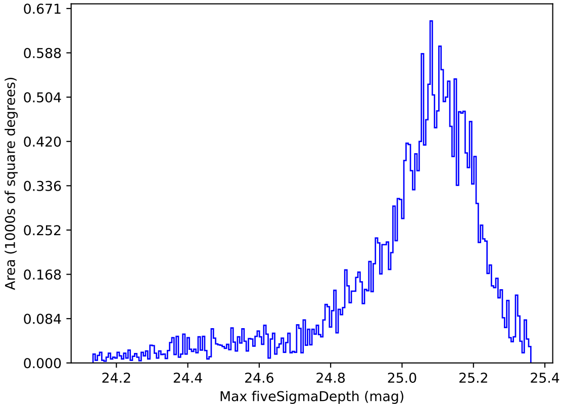
ddf_half_v3.4_10yrs All sky g band: Max fiveSigmaDepth
