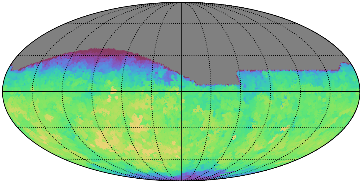
ddf_half_v3.4_10yrs All sky all bands: Max fiveSigmaDepth
