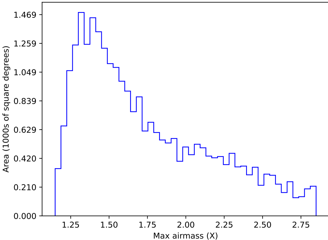
ddf_half_v3.4_10yrs Yr 1 z band: Max airmass
