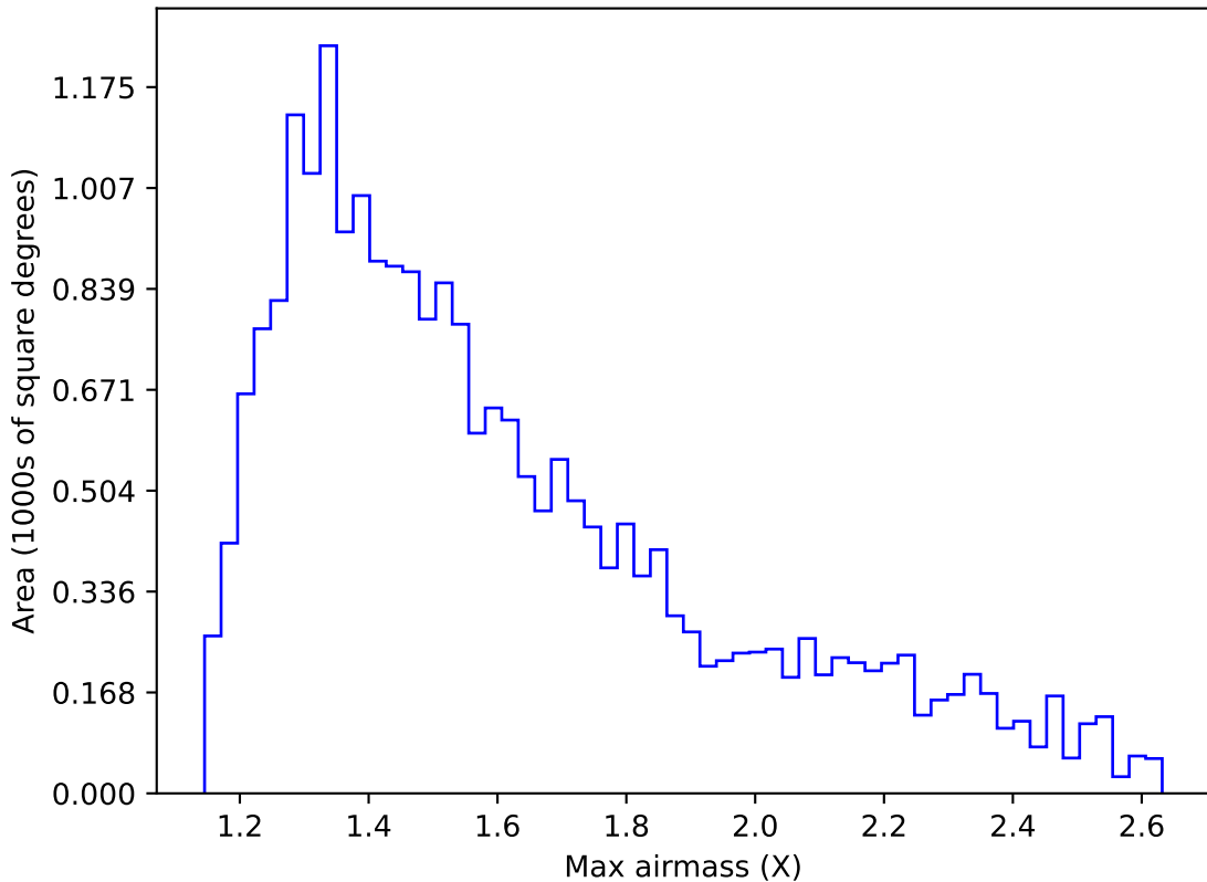
ddf_half_v3.4_10yrs Yr 1 y band: Max airmass
