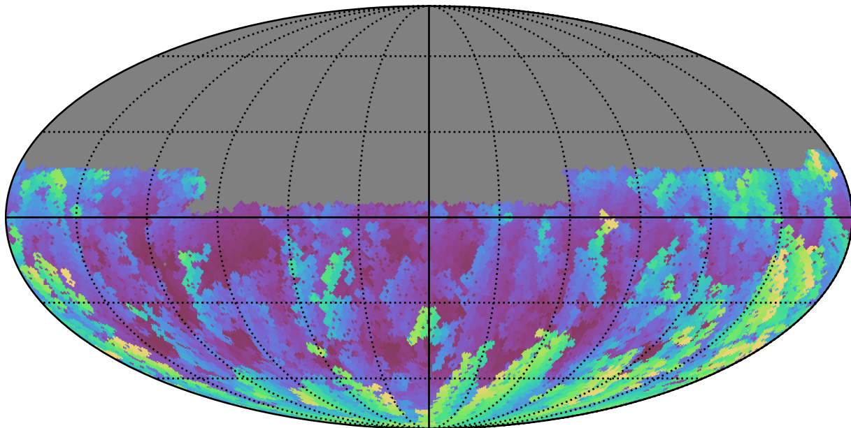
ddf_half_v3.4_10yrs Yr 1 u band: Max airmass
