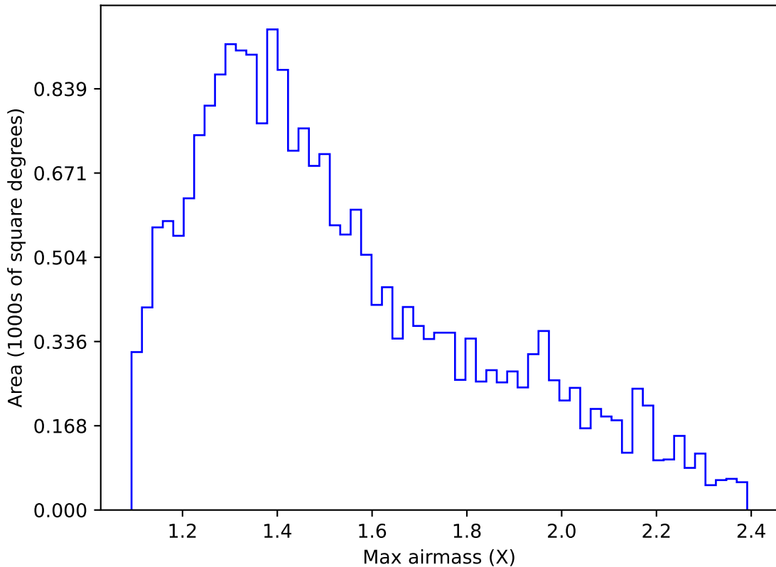
ddf_half_v3.4_10yrs Yr 1 u band: Max airmass
