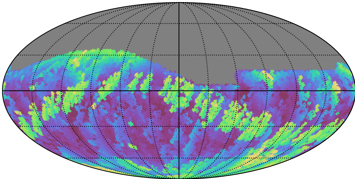
ddf_half_v3.4_10yrs Yr 1 r band: Max airmass
