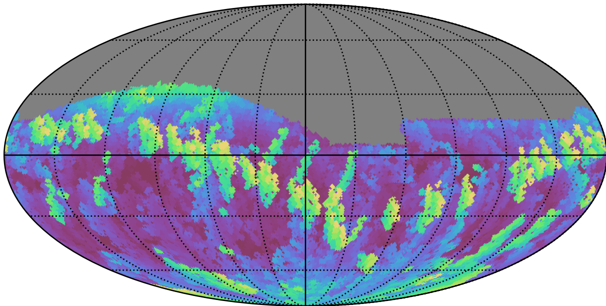
ddf_half_v3.4_10yrs Yr 1 i band: Max airmass
