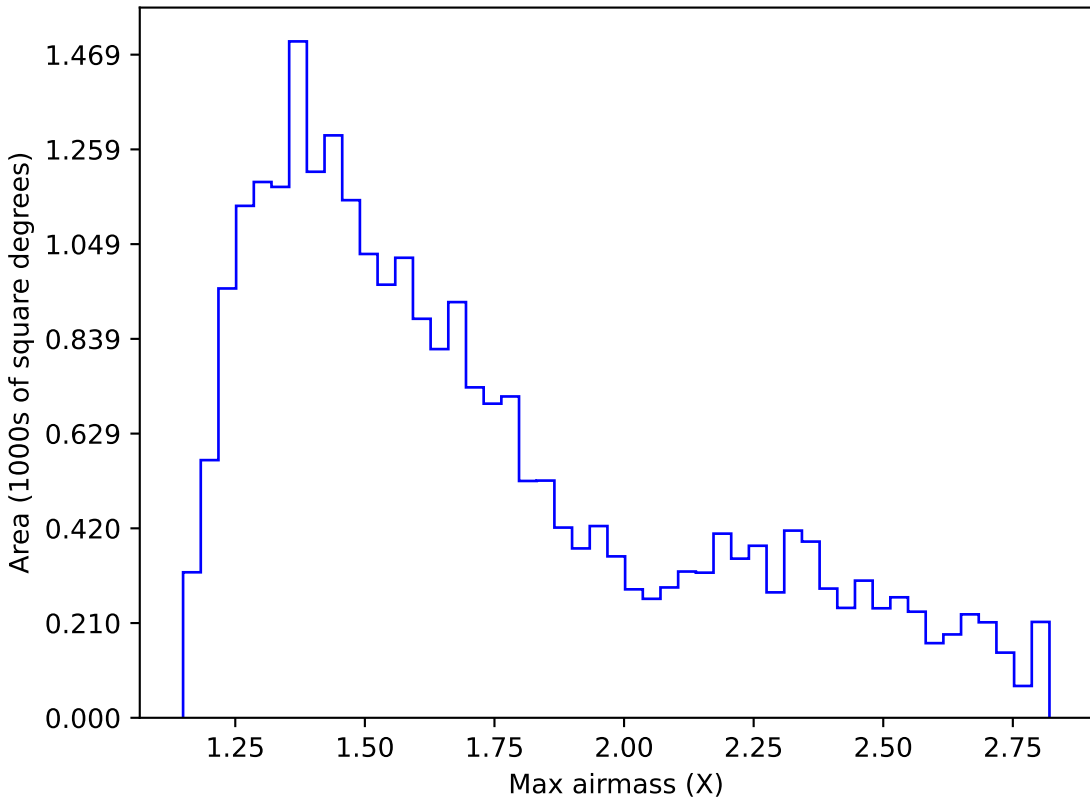
ddf_half_v3.4_10yrs Yr 1 i band: Max airmass
