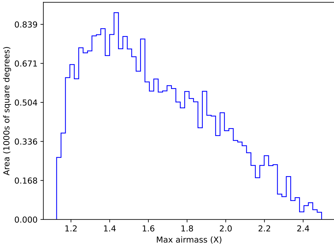
ddf_half_v3.4_10yrs Yr 1 g band: Max airmass
