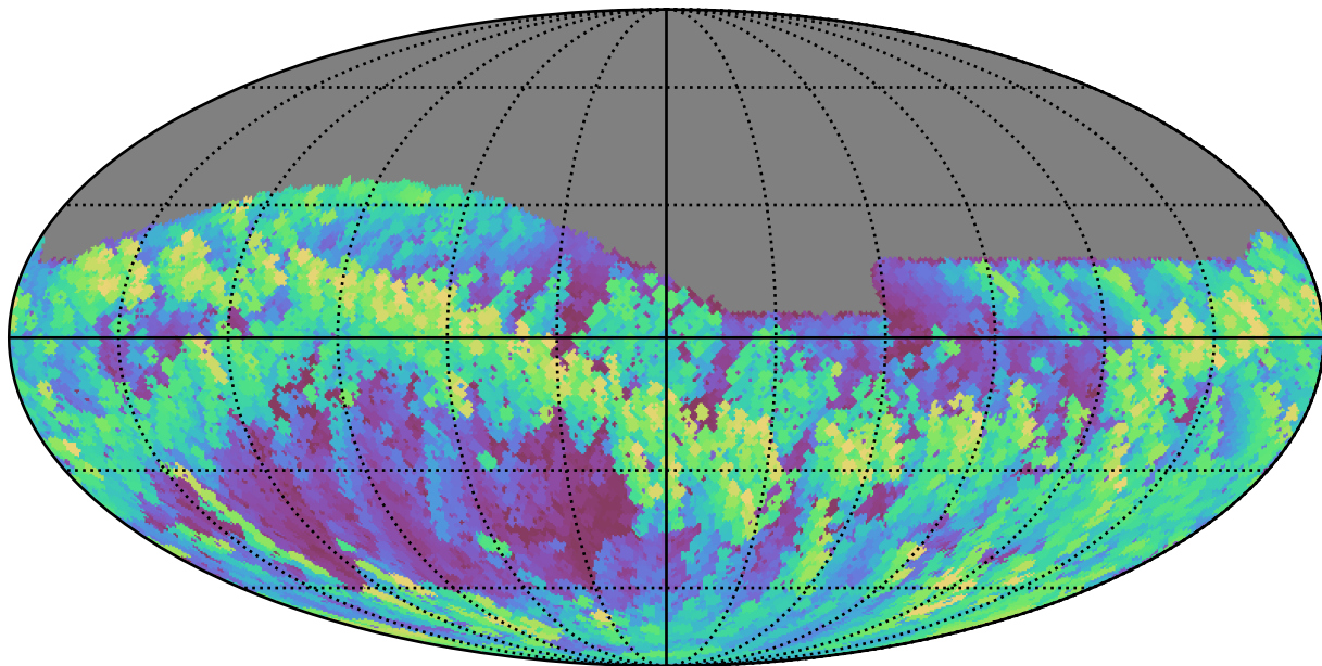
ddf_half_v3.4_10yrs Yr 1 all bands: Max airmass
