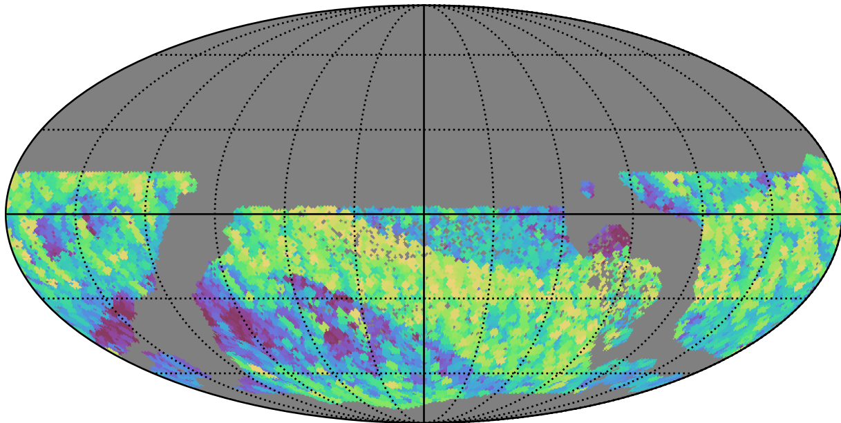
ddf_half_v3.4_10yrs WFD z band: Max airmass
