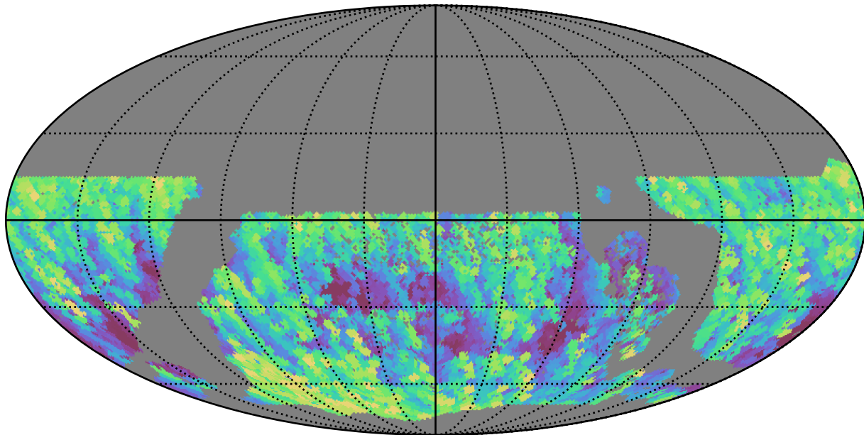
ddf_half_v3.4_10yrs WFD y band: Max airmass
