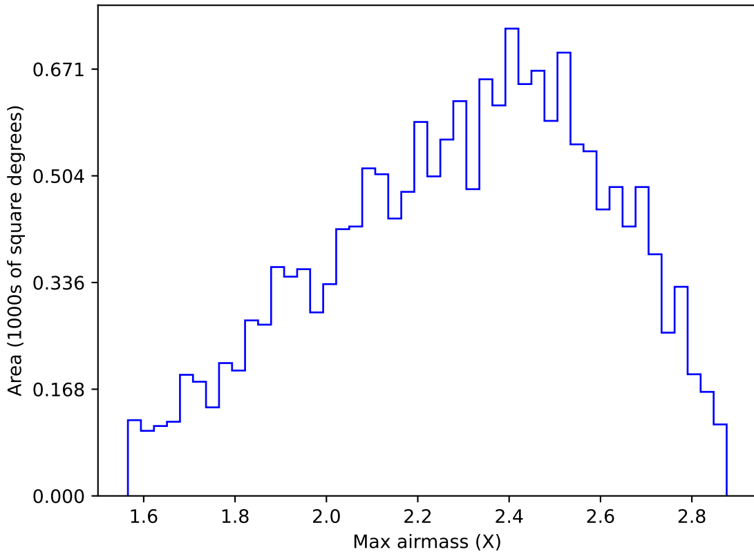
ddf_half_v3.4_10yrs WFD y band: Max airmass
