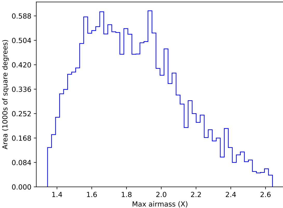
ddf_half_v3.4_10yrs WFD u band: Max airmass
