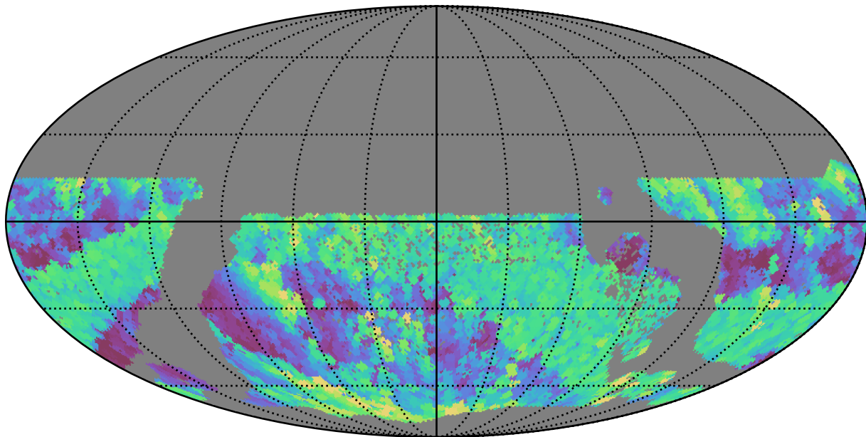
ddf_half_v3.4_10yrs WFD r band: Max airmass
