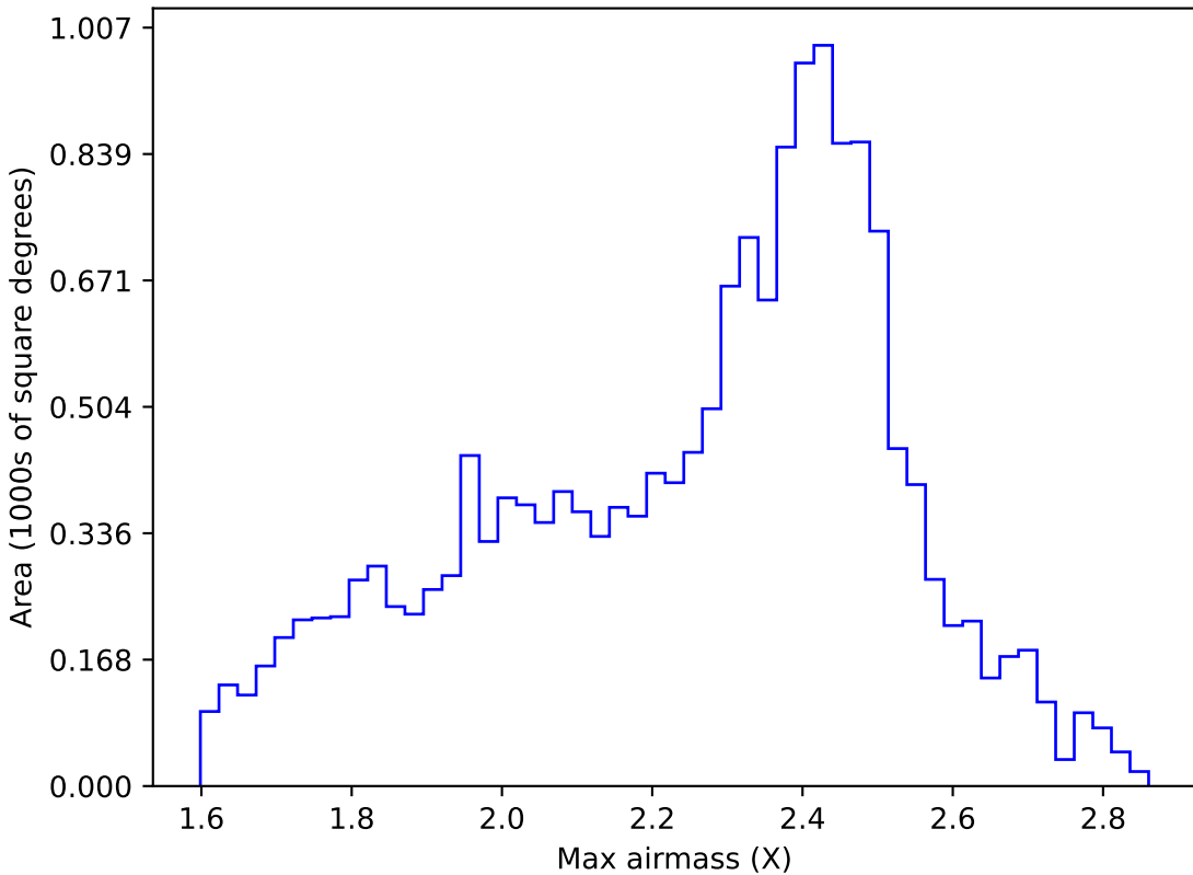
ddf_half_v3.4_10yrs WFD r band: Max airmass
