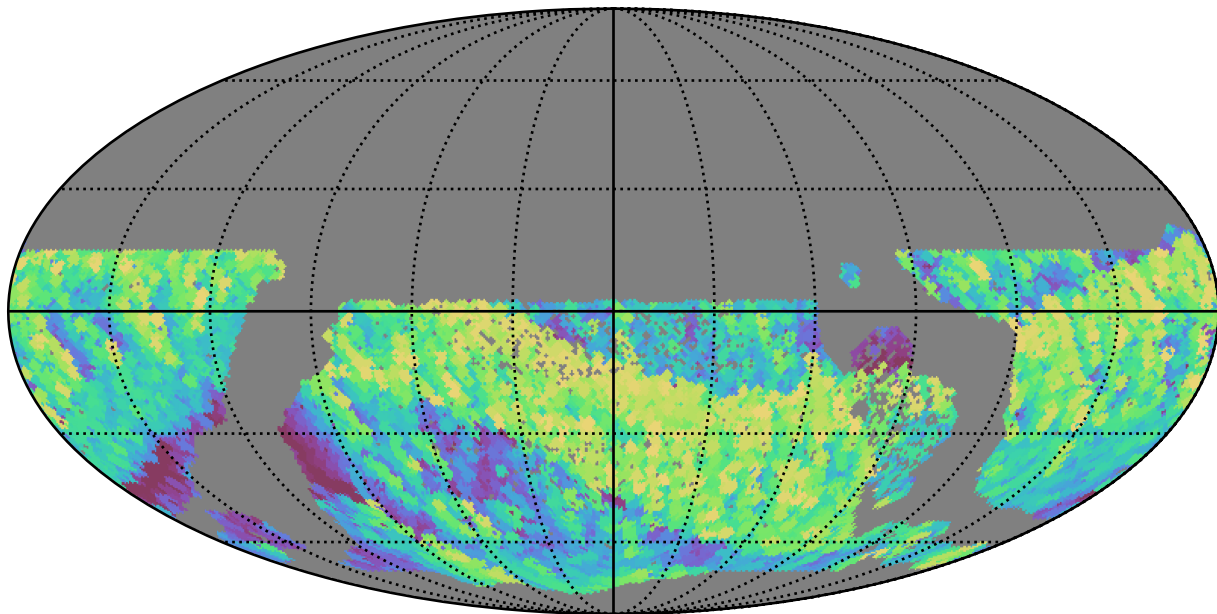
ddf_half_v3.4_10yrs WFD i band: Max airmass
