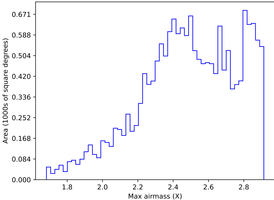
ddf_half_v3.4_10yrs WFD i band: Max airmass
