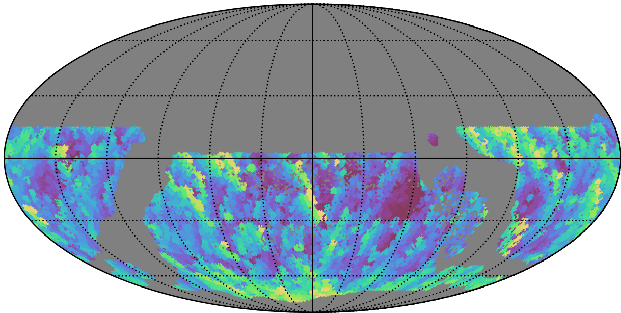
ddf_half_v3.4_10yrs WFD g band: Max airmass
