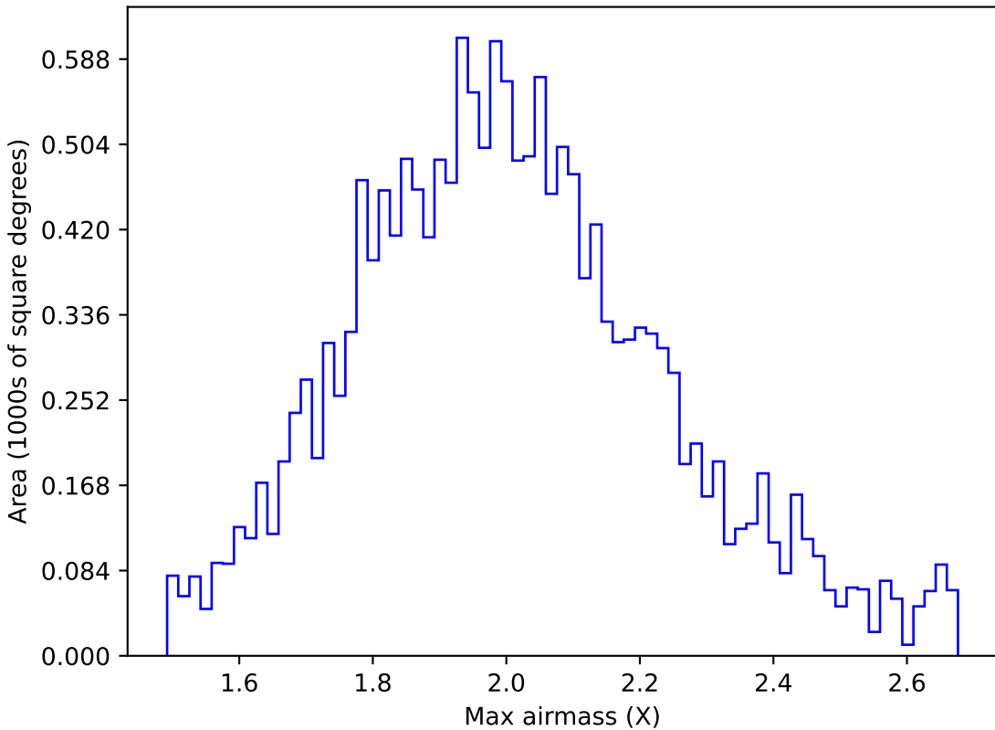
ddf_half_v3.4_10yrs WFD g band: Max airmass
