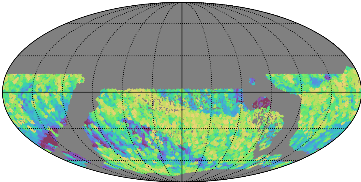
ddf_half_v3.4_10yrs WFD all bands: Max airmass
