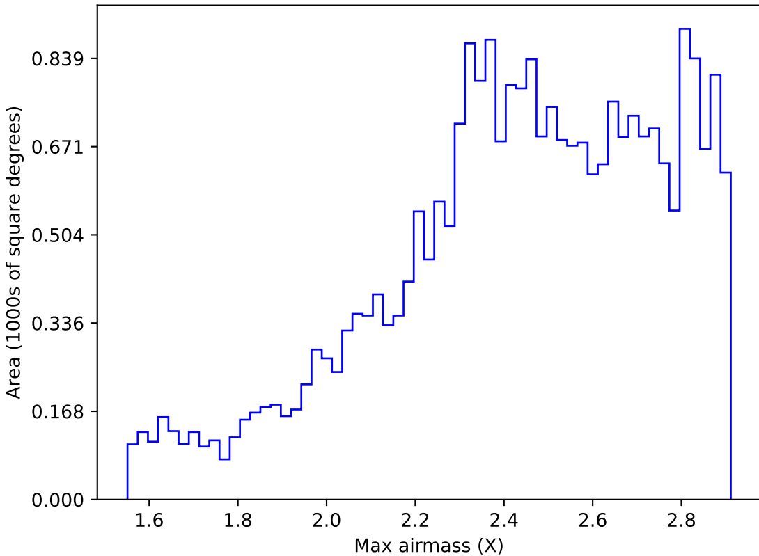
ddf_half_v3.4_10yrs All sky z band: Max airmass
