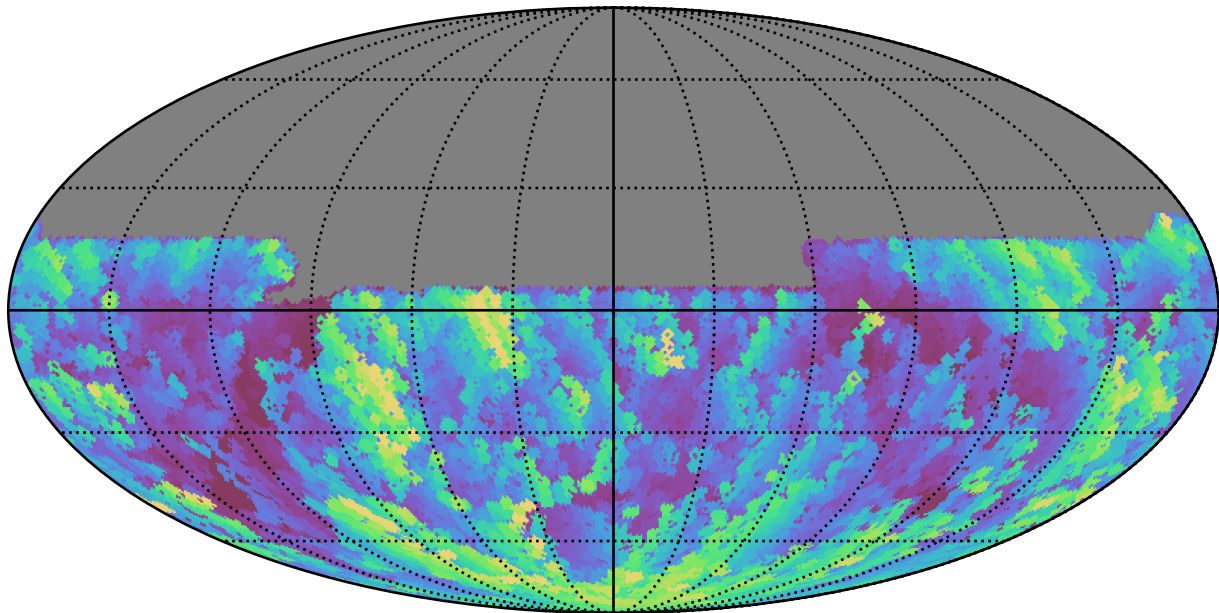
ddf_half_v3.4_10yrs All sky u band: Max airmass
