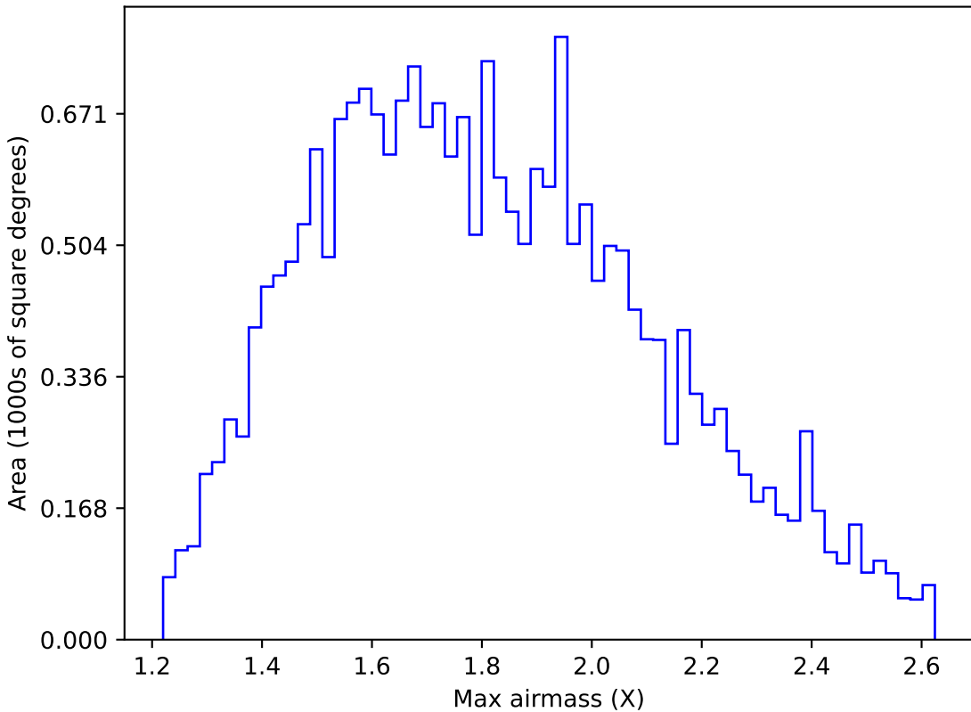
ddf_half_v3.4_10yrs All sky u band: Max airmass
