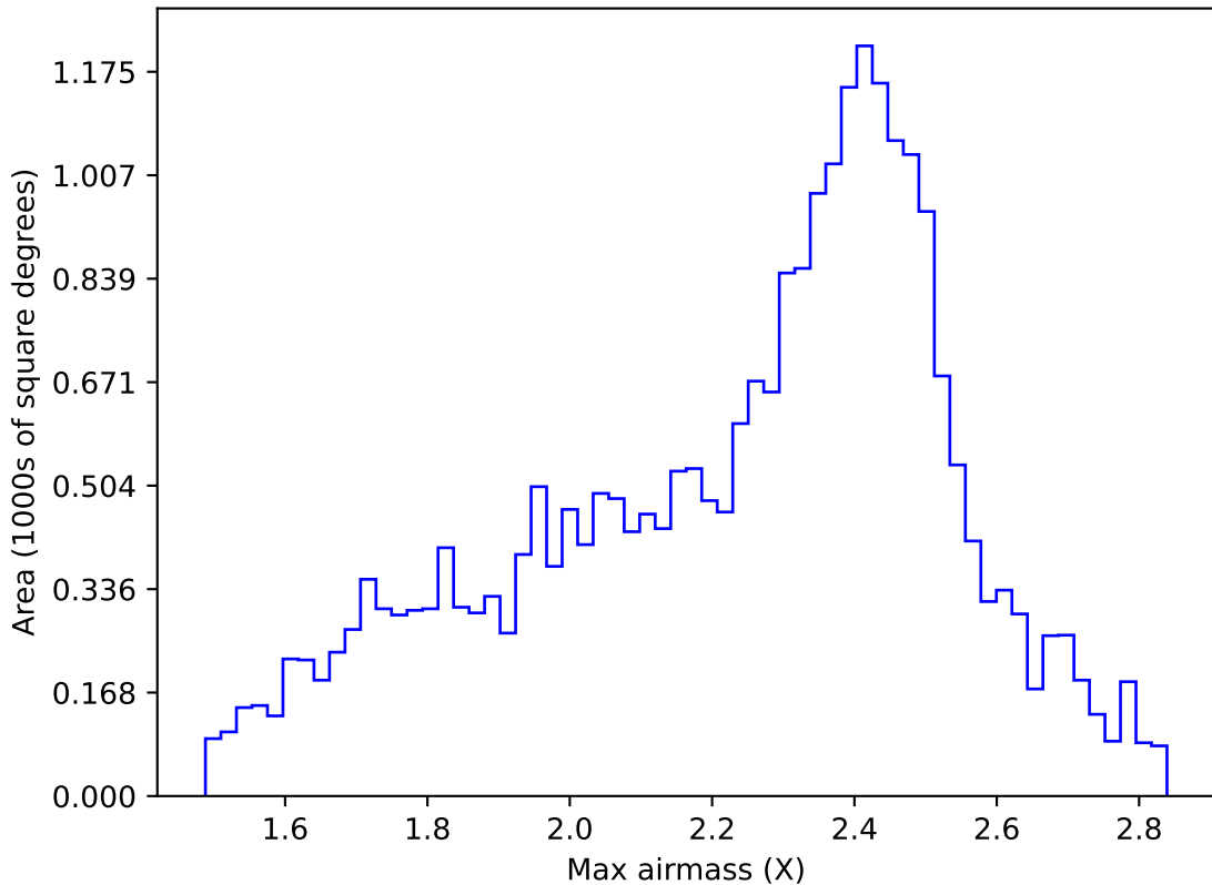
ddf_half_v3.4_10yrs All sky r band: Max airmass
