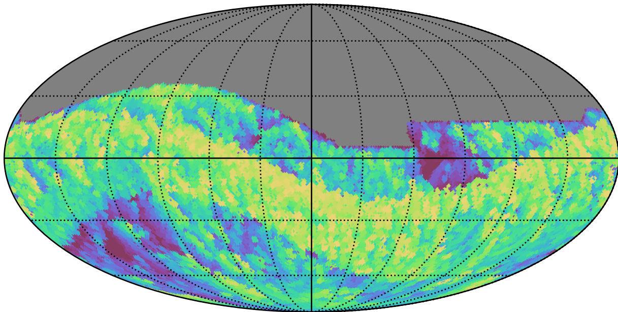
ddf_half_v3.4_10yrs All sky i band: Max airmass
